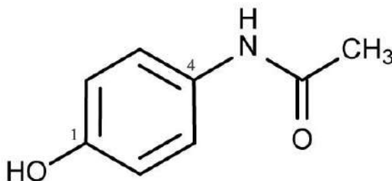
Figure 1. Structure of acetaminophen (N-Acetyl-4-aminophenol). The phenolic structure with a substituent at the para position relative to the hydroxyl group allows acetaminophen to react with reactive species and possesses antioxidant activity. Cited from (Blough and Wu, 2011).
