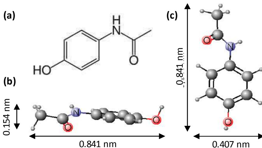
Figure 2. Molecular structure of acetaminophen. (a) General structure (b) and (c) special arrangement of the atoms with molecular dimensions.
